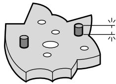
Press-fitting pins Height & pressure control
