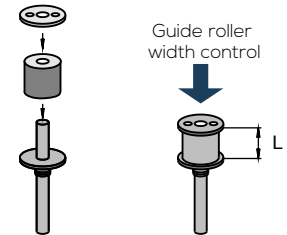
Guide roller press fitting for video tape Guide roller width control
