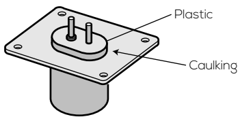
Caulking for electro plug Caulking without damaging plastic part
