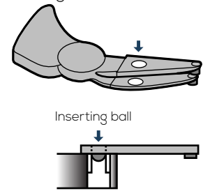
Attaching disk drive reading arm
