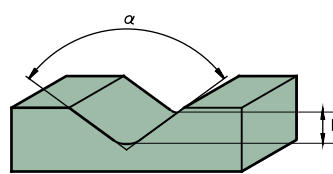
V-groove treatment for oil pressure parts Depth L control
