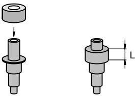
Inserting electronic parts Pressure control for L distance
